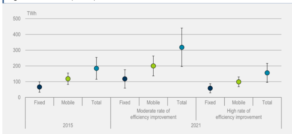
Figure 5.3 Electricity use by internet data transmission networks
