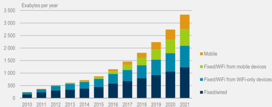
Figure 5.4 Global IP traffic by access mode
